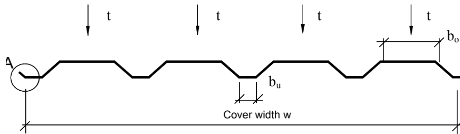
Figure B1.2: Measuring points for sheet thickness t and deviation of sidelap D
